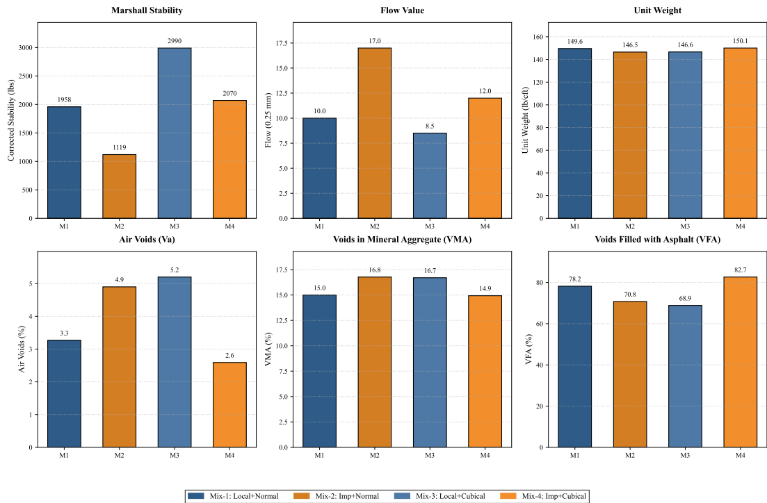
Figure 4.5: Performance assessment of the four bituminous mix variants across Marshall stability, flow, and volumetric parameters.
